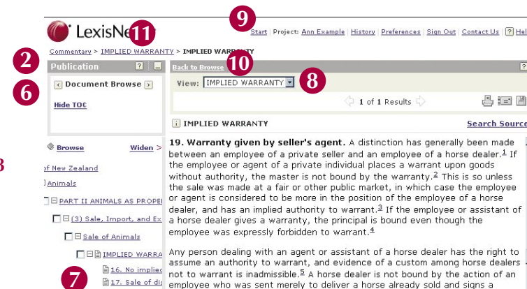
Figure 3: Document View
