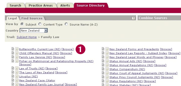
Figure 1: Source Directory
